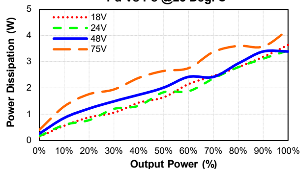
EC5SBW-48D15 Pd Vs Po @25 Deg. C
