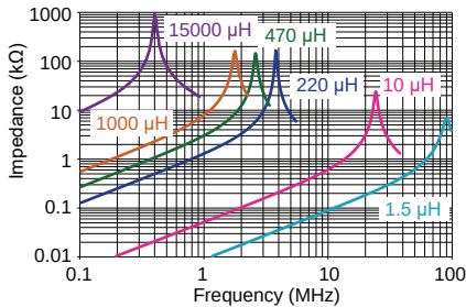
Typical |Z| vs Frequency (f)
