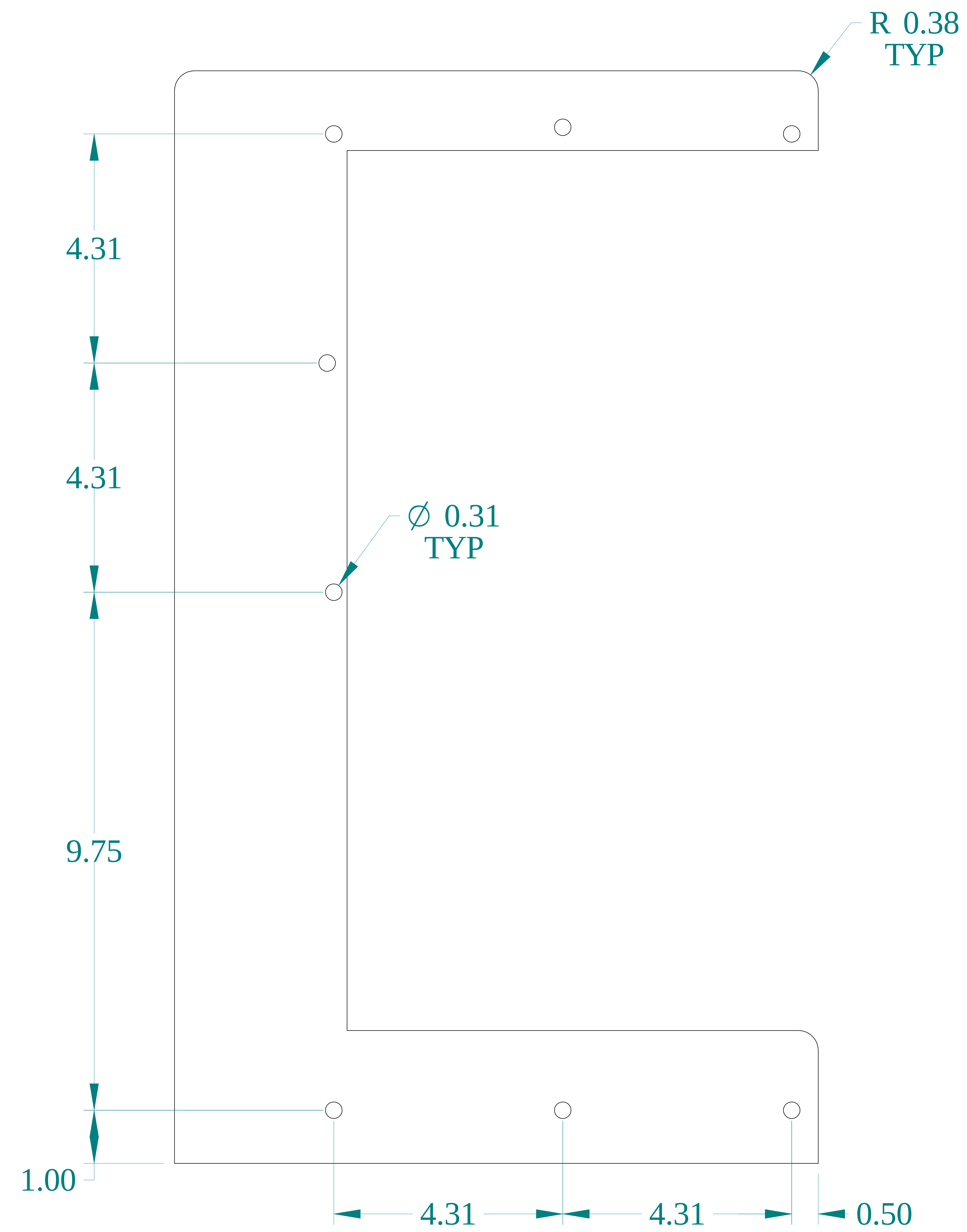
FRONT VIEW
