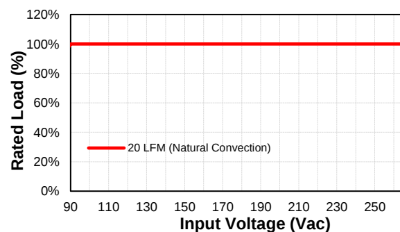
TR60M Input Voltage Derating Curve
