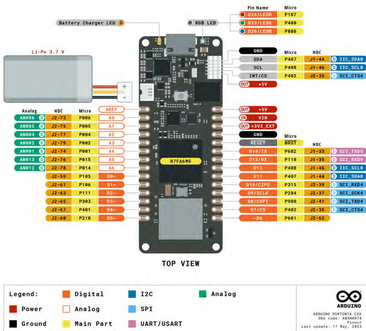
Figure 1. Portenta C33 pinout (MKR-styled connectors)
