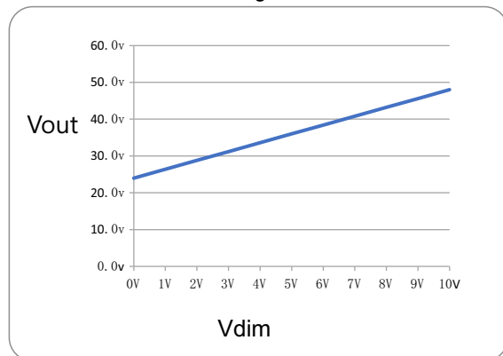
Dimming Curve
