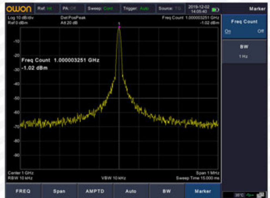
frequency counter
