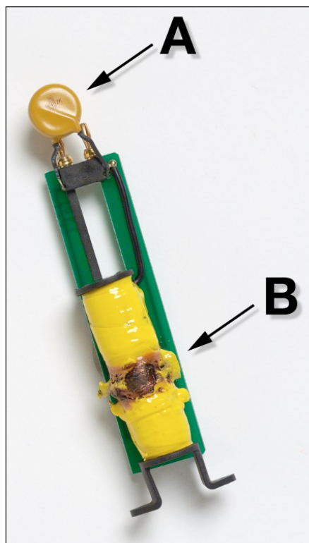
Figure 1: This solenoid tester experienced a catastrophic failure after receiving an impulse. Even with an MOV (metal oxide varistor) (see A), the unit will still self-destruct from overheating (see B).
