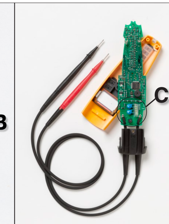
Figure 2: Current-limiting resistors (see C) protect this electronic tester which results in a predictable failure mechanism when the tester is exposed to electrical impulses.
