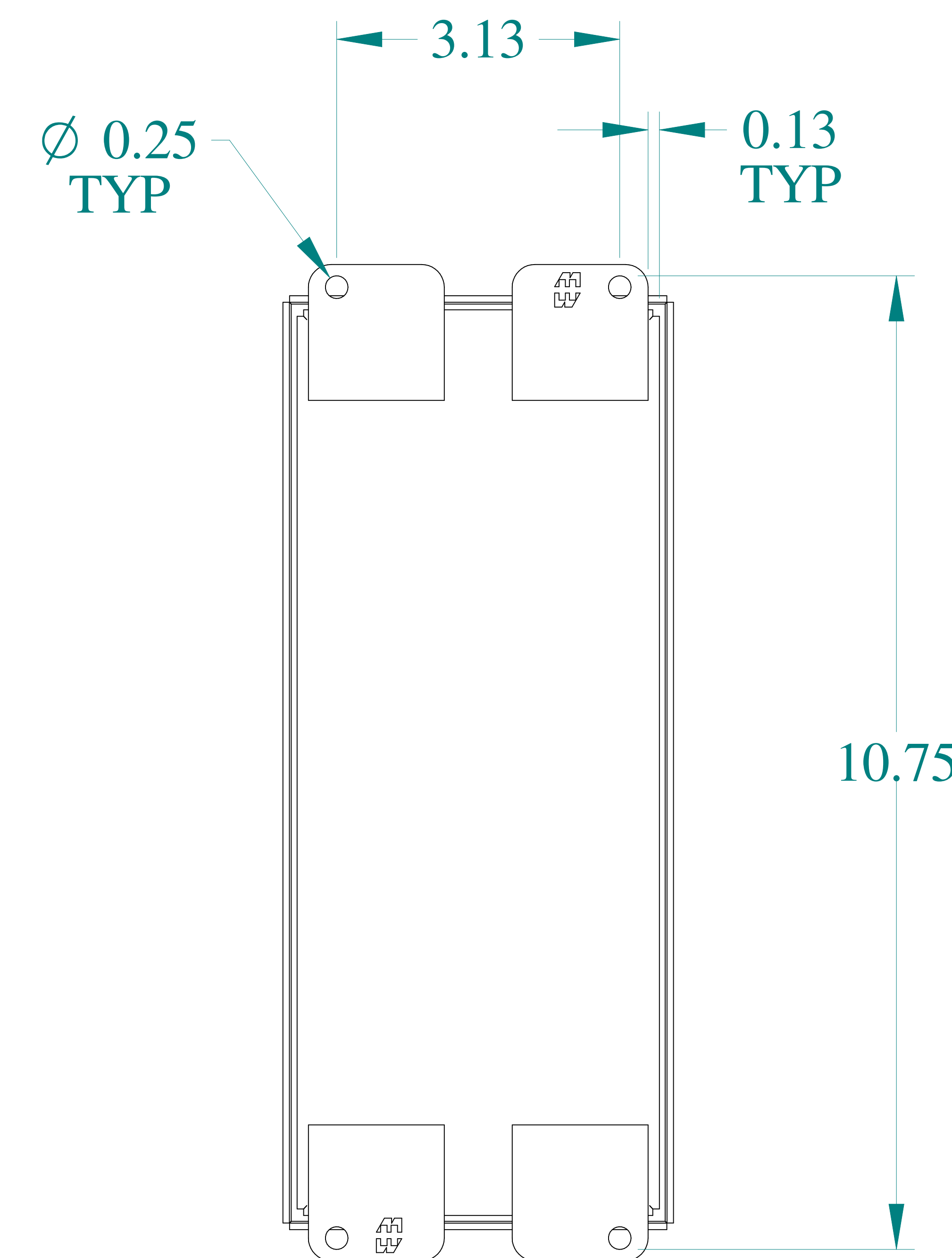
BACK VIEW
