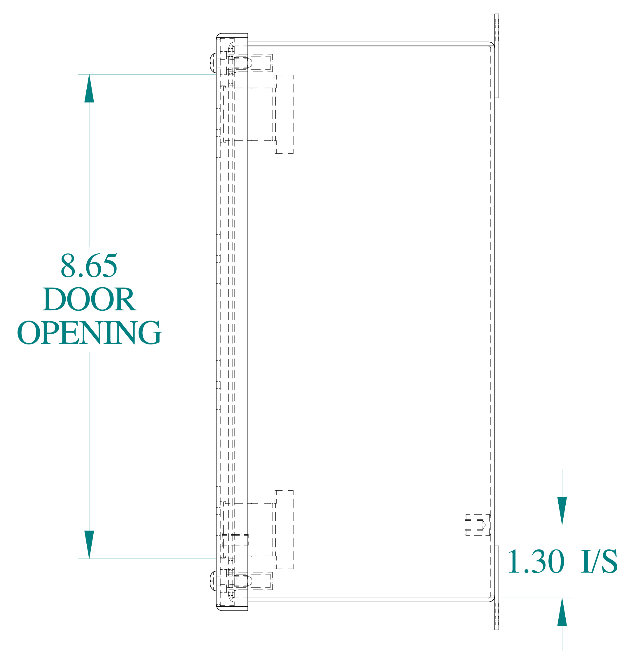
SIDE VIEW
