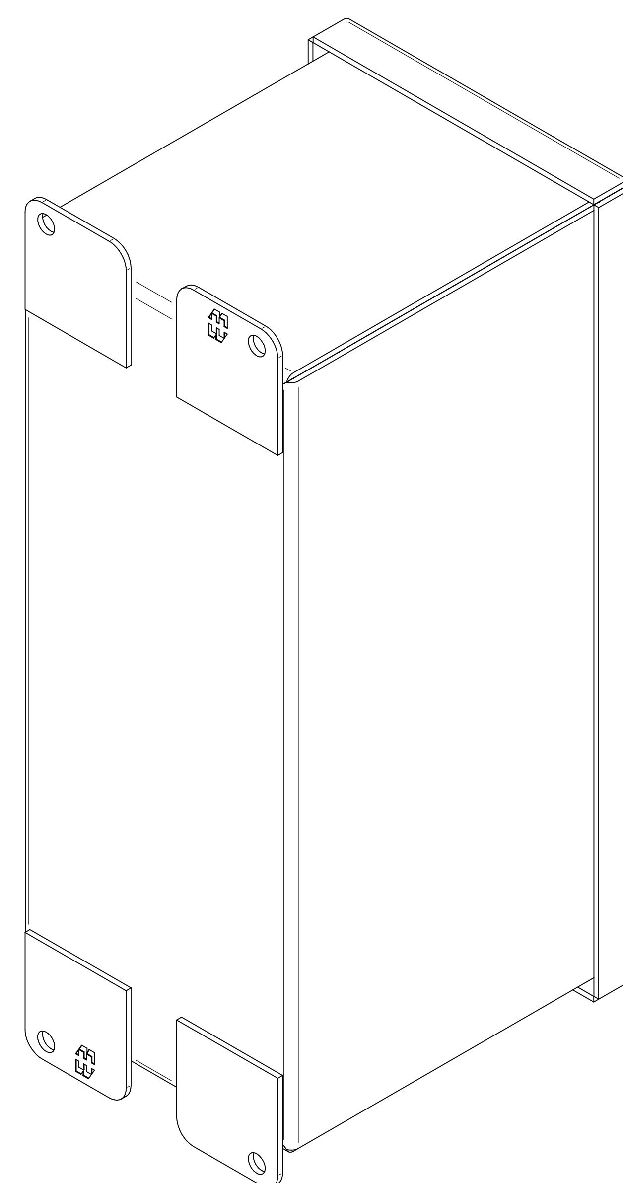
ISOMETRIC VIEWS
