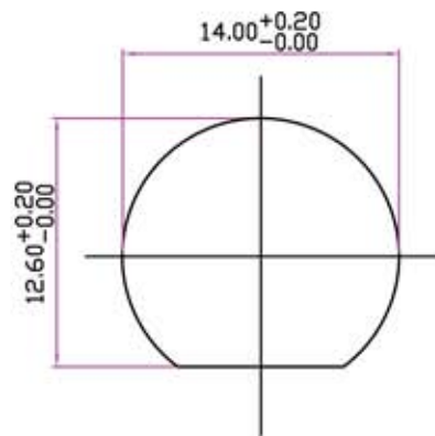
PANEL CUT-OUT
