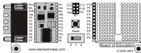
Figure 1-50 Switching Off the Power for the Board of Education Rev C
