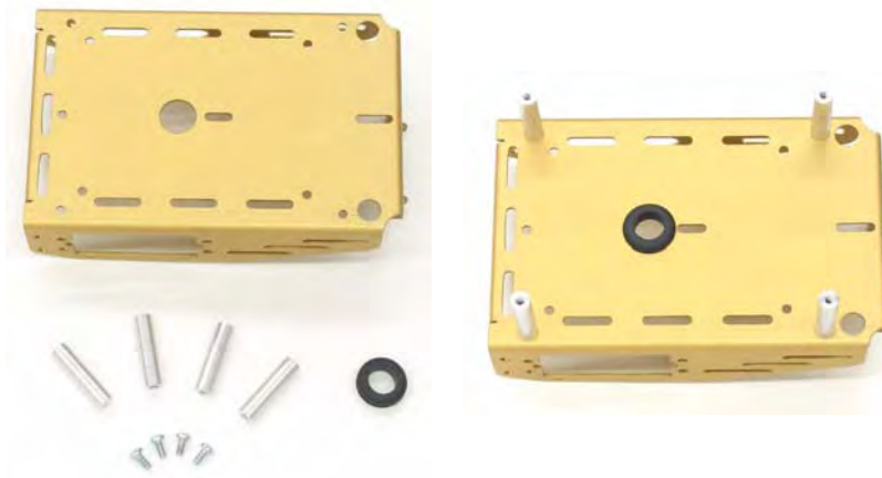
Figure 3-2 Chassis and Topside Hardware
