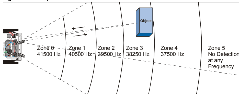
Figure 8-2: Frequencies and Zones for the Boe-Bot
