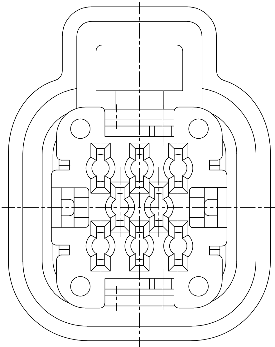
BOTTOM VIEW WITH LOCKING WEDGE
