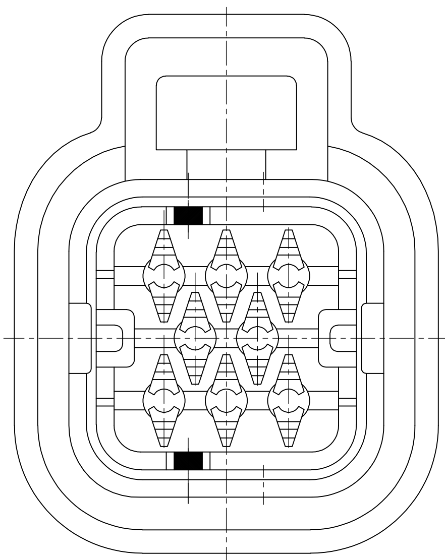
KEY LOCATION FOR 776281-1 SCALE 4:1
