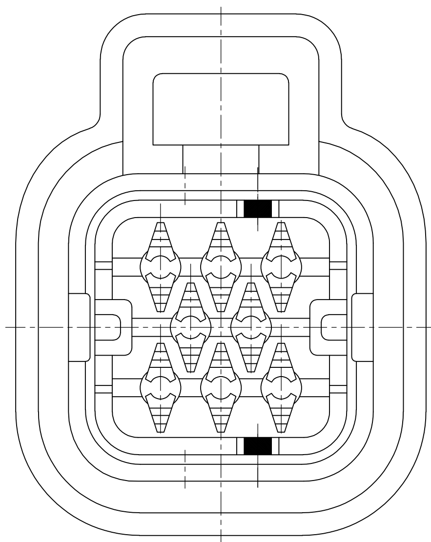
KEY LOCATION FOR 776281-2 SCALE 4:1
