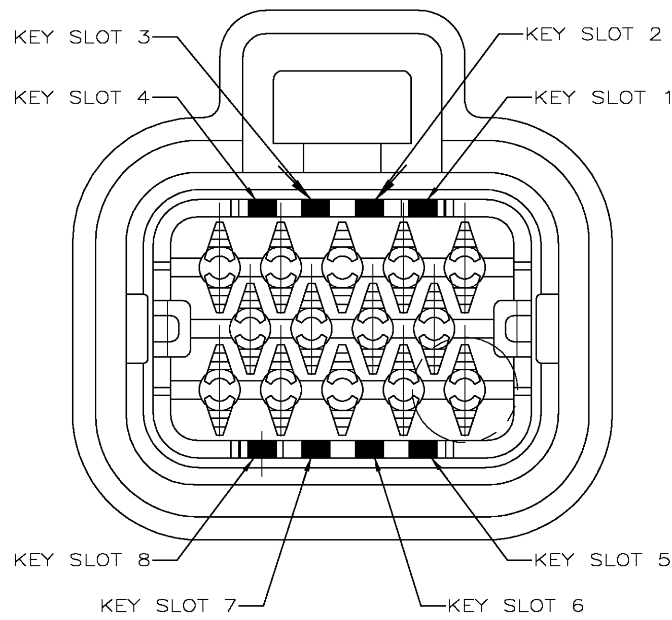
KEY SLOT LOCATION SCALE 4:1
