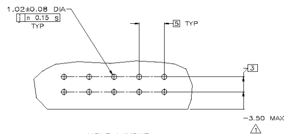
HOLE LAYOUT
