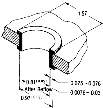
PC Board Hole Dimension
