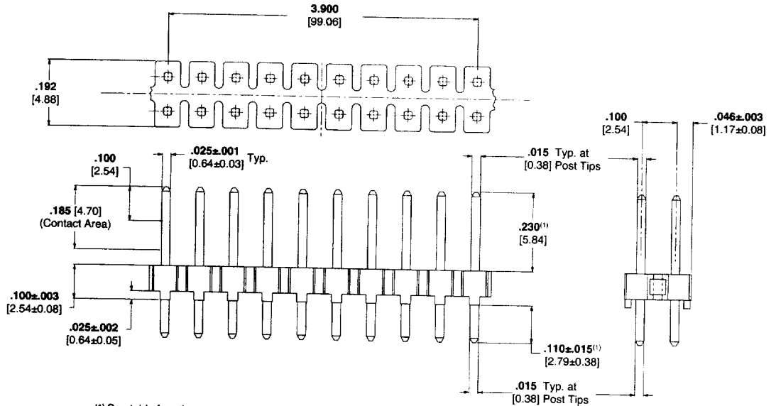
Standard Breakaway-to-Reeled Header Conversion Chart (Vertical)
