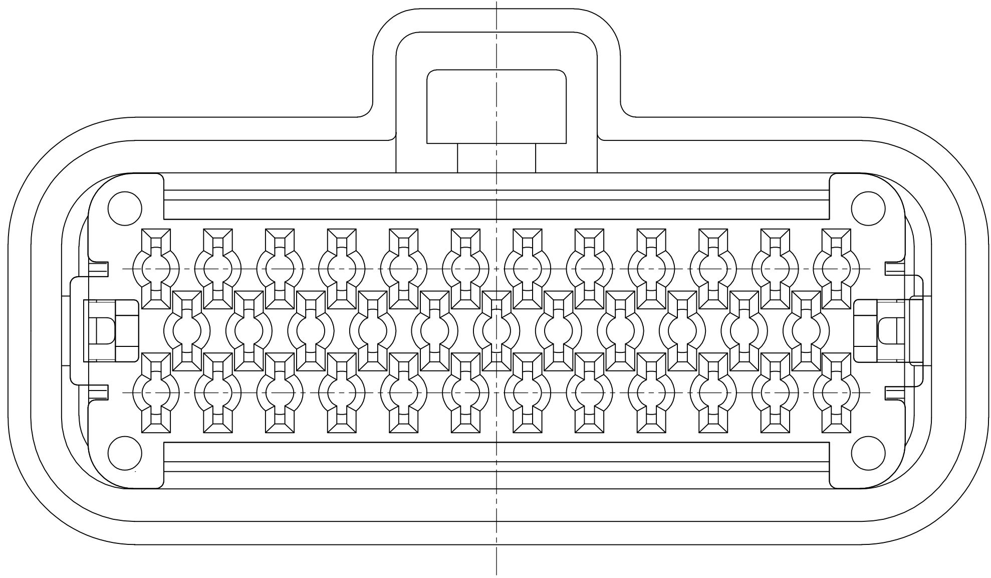
BOTTOM VIEW WITH LOCKING WEDGE
