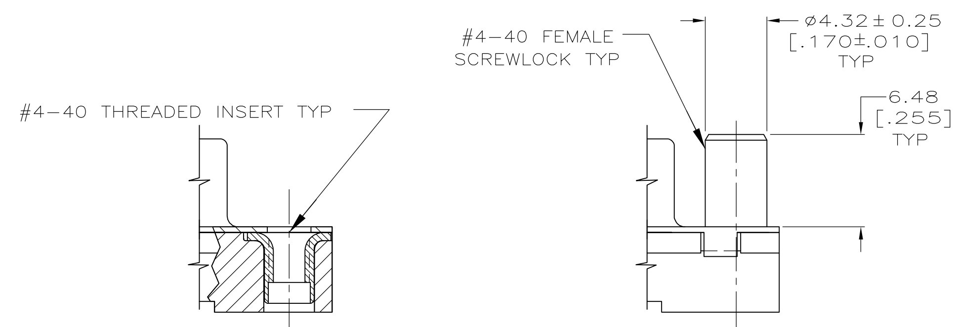
DETAIL E
