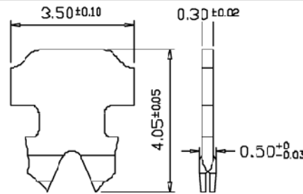
“2” : 2 PRONGS FOR SOLID WIRE(SS)
