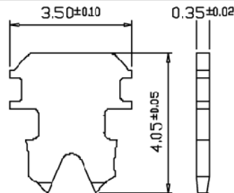
“ ” : 2 PRONGS FOR STRANDED WIRE
