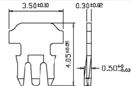
“3” : 3 PRONGS FOR SOLID WIRE(S)
