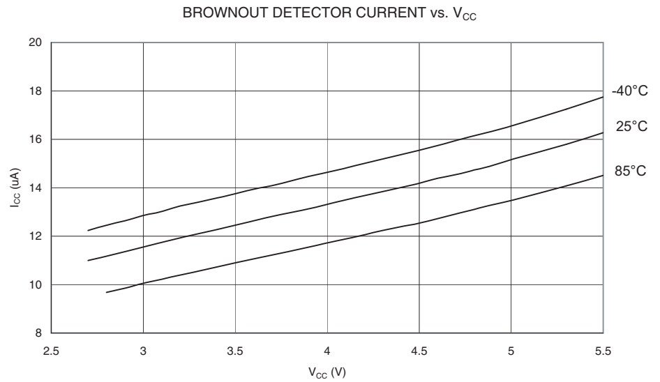
Figure 206. Brownout Detector Current vs. V_{CC}
