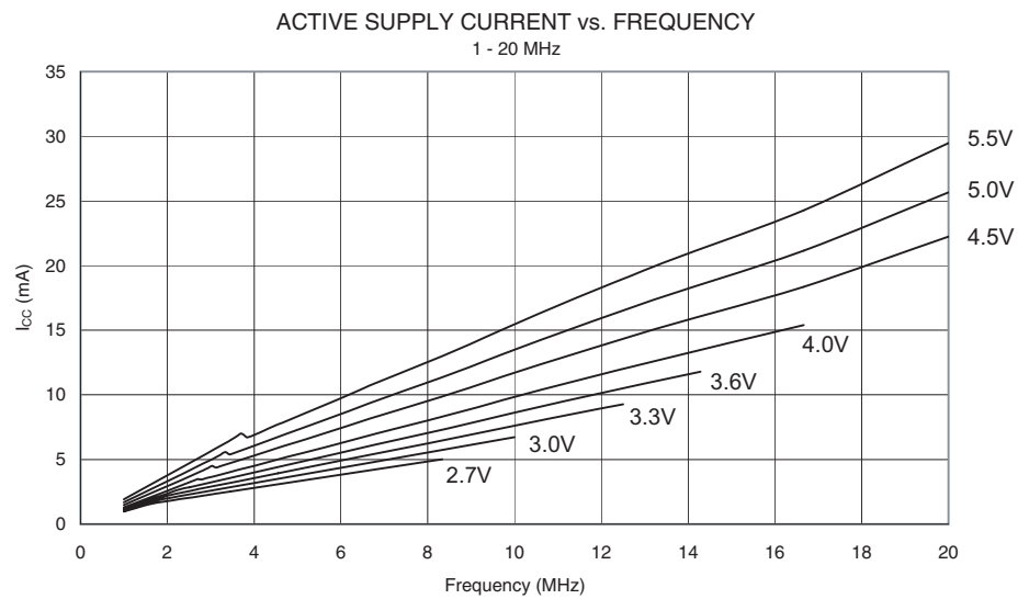
Figure 150. Active Supply Current vs. Frequency (1 - 20 MHz)
