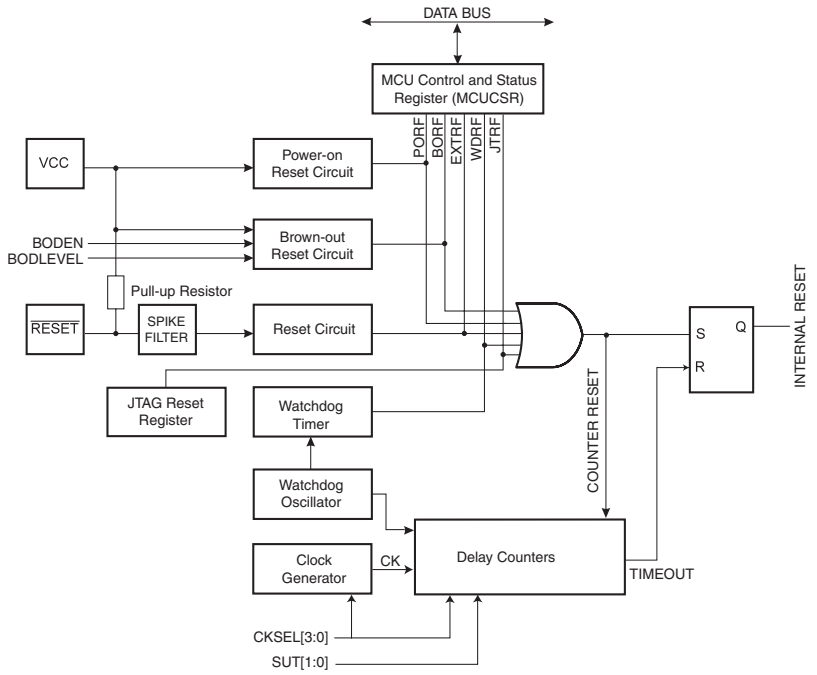
Figure 15. Reset Logic
