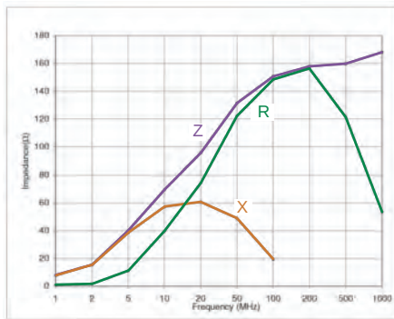
Z-f Charecteristics
