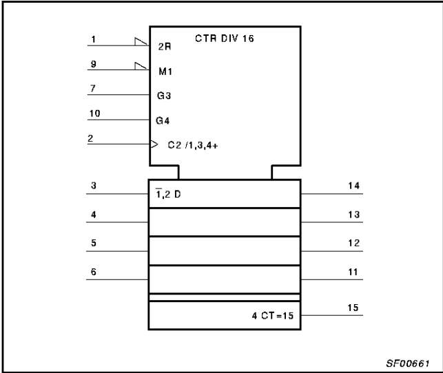
74F163A LOGIC SYMBOL (IEEE/IEC)
