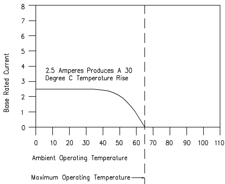
Figure 4 Current Rating
