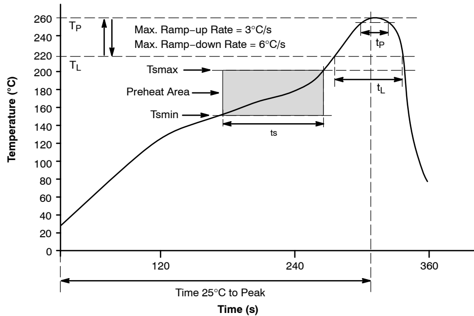
Figure 20. Reflow Profile
