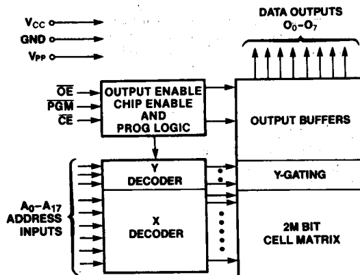
Figure 1. Block Diagram
