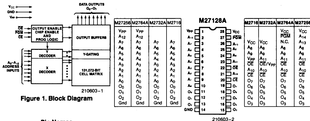
Figure 2. Pin Configurations
