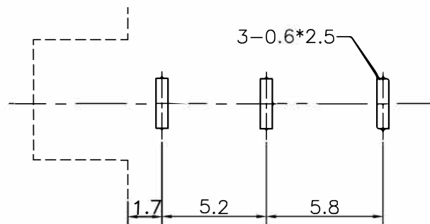
P.C.B. HOLE LAYOUT (BOTTOM VIEW)
