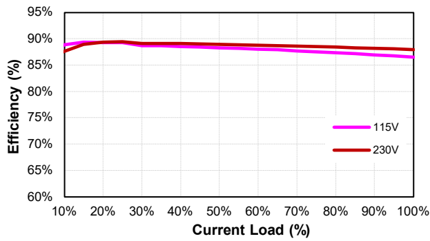
TRH70A180 (Eff Vs Io)
