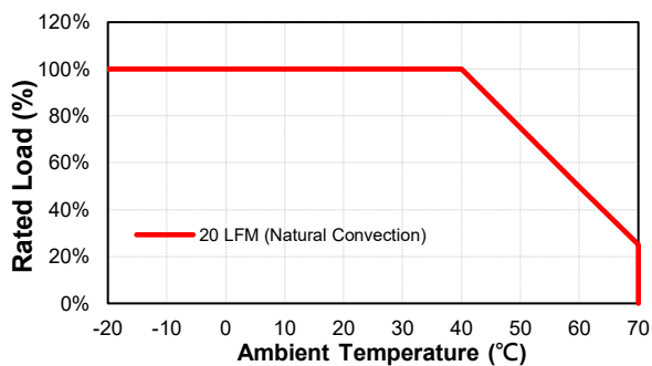
TRH70A Derating Curve
