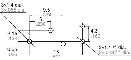
PC board pattern (Bottom view)
