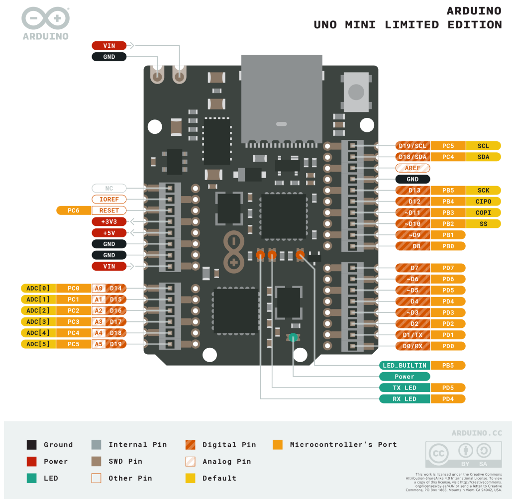
Pinout
