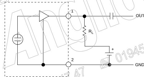
Schematic
