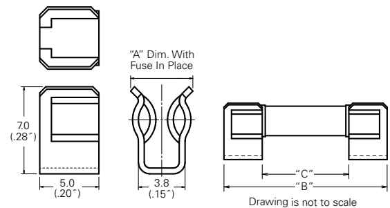
111 505 Device Dimensions
