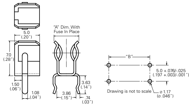
111 501 / 111 506 Device Dimensions
