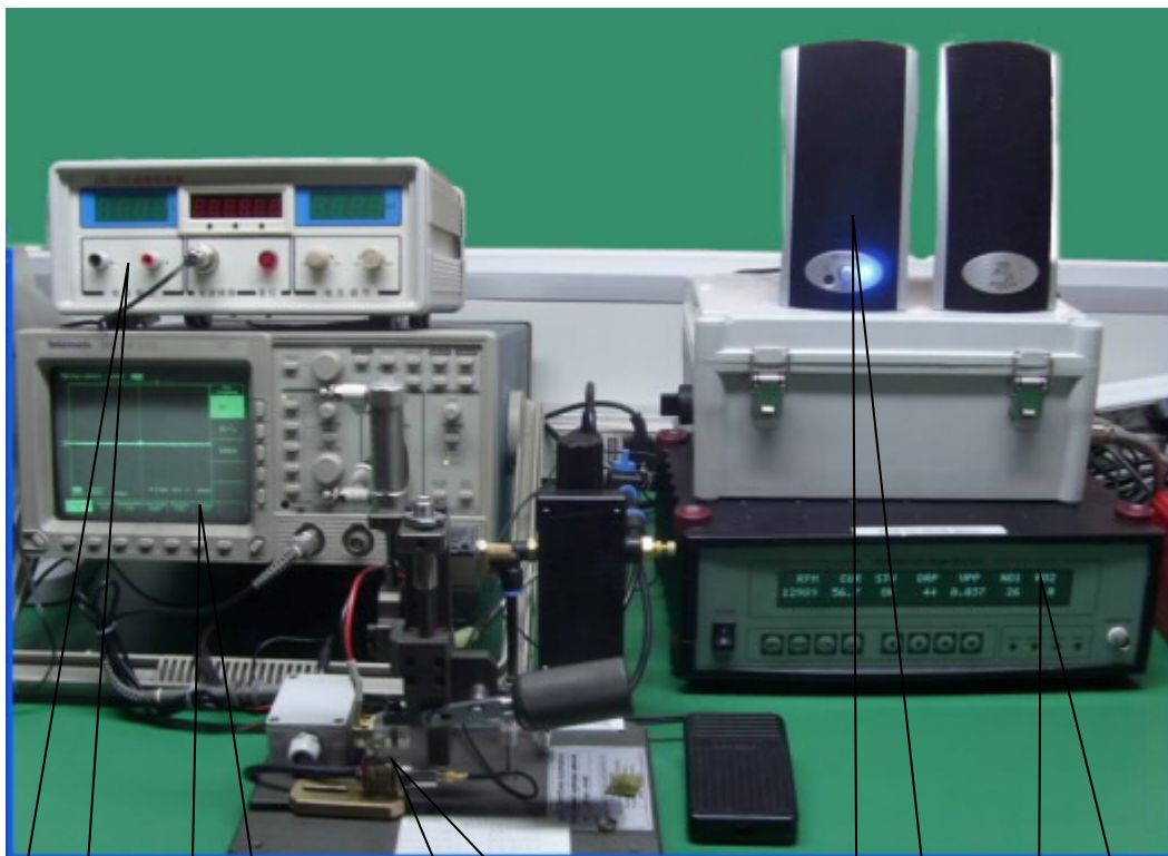
马达安放装置 Test Jig (for Clamping the Motor in Place)
