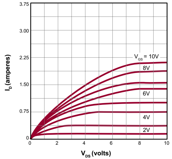
Saturation Characteristics
