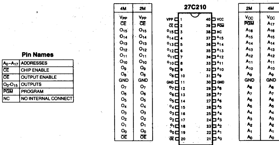
Figure 2. DIP Pin Configuration
