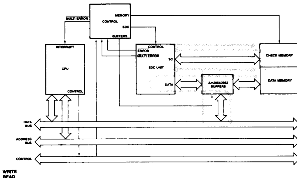
Figure 12. Correct-Always Configuration
