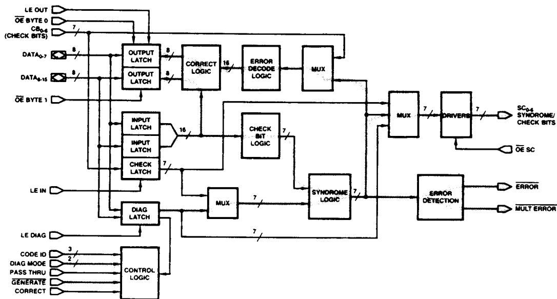
Figure 4. Diagnostic Detect and Correct Data Path
