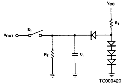
Figure 25. Normal Outputs
