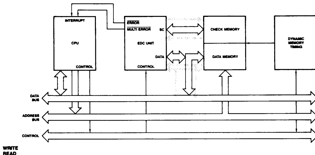
Figure 11. Check-Only Configuration
