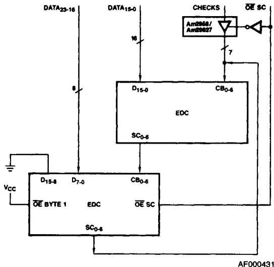
Figure 18. 24-Bit Configuration
