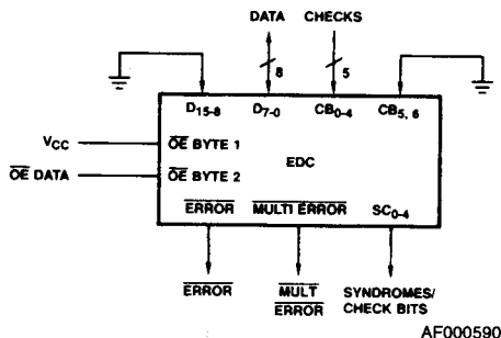
Figure 17. 8-Bit Configuration
