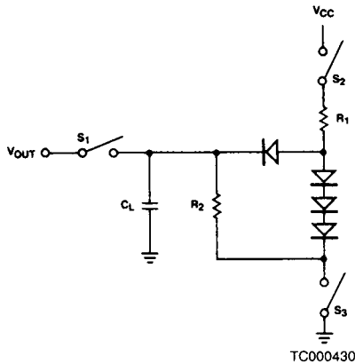
Figure 24. Three-State Outputs
