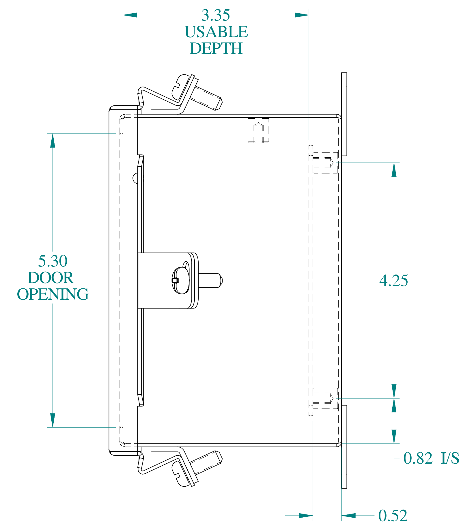
SIDE VIEW
