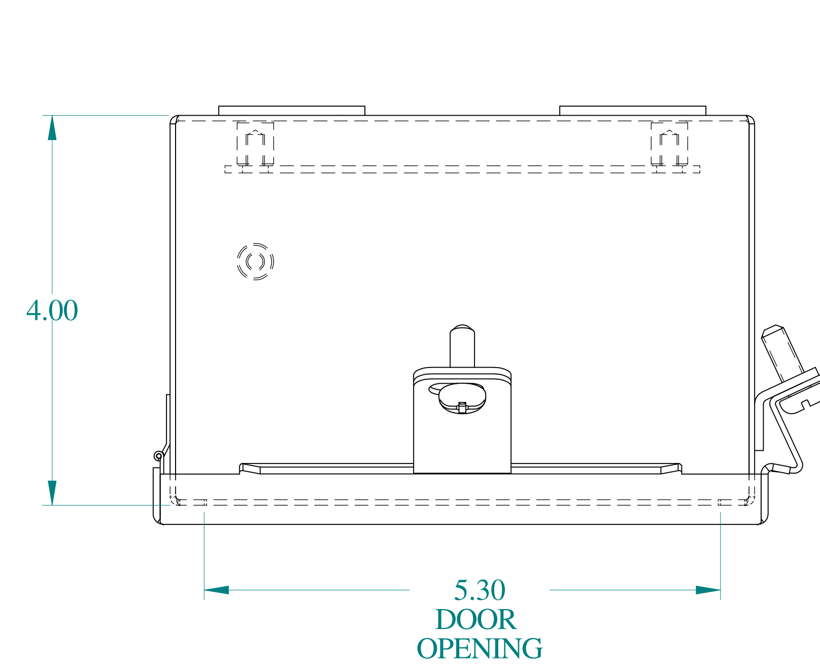
TOP VIEW
