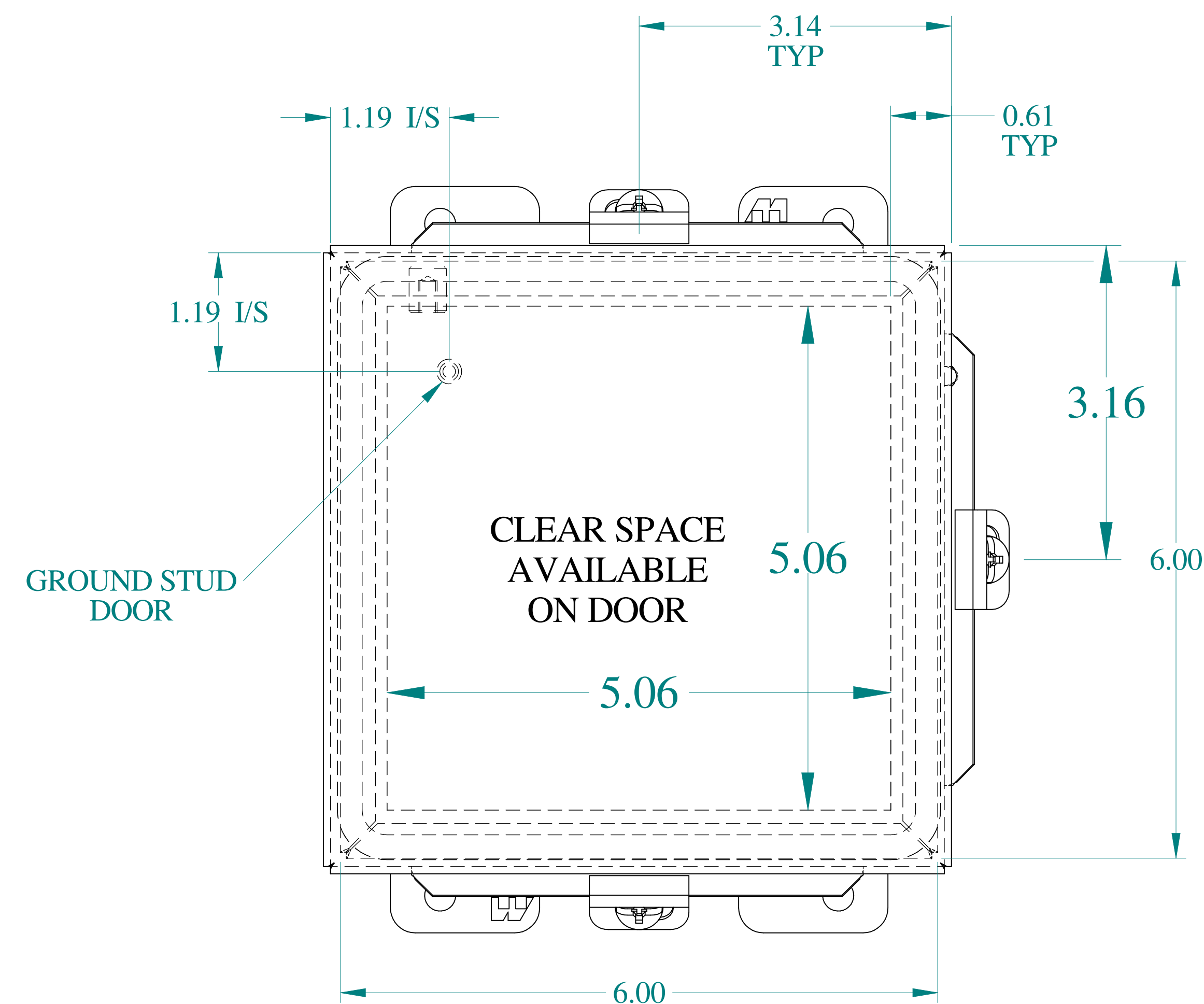
FRONT VIEW
