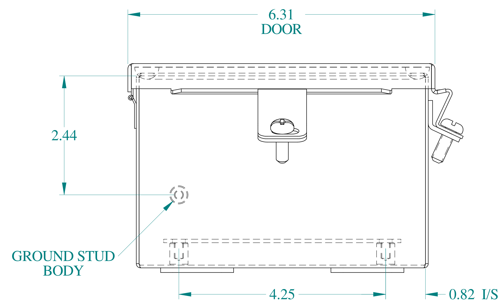
BOTTOM VIEW
