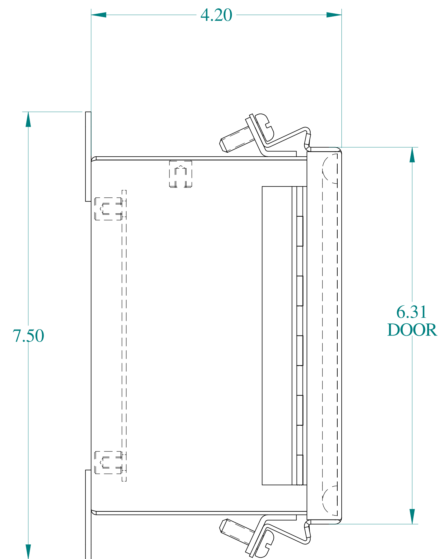
SIDE VIEW
