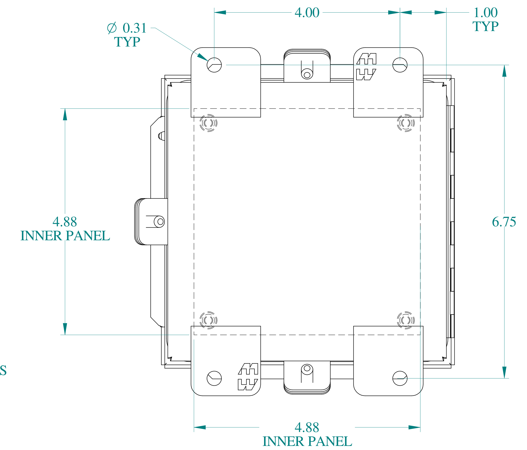
BACK VIEW
