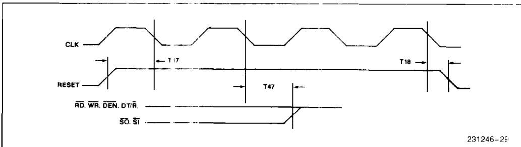
Figure 28. RESET Timing
