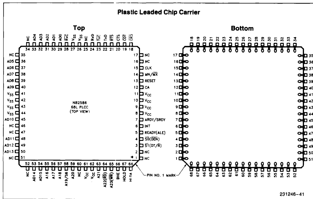
Figure 2. 82586 Pinout Diagrams
