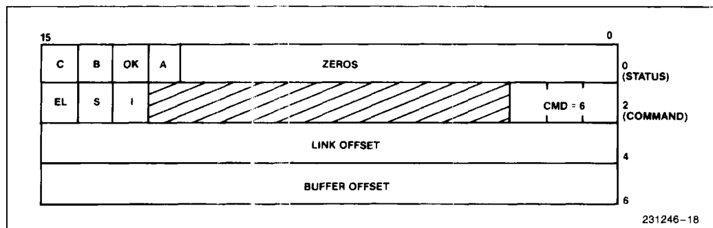
Figure 13. The DUMP Command Block
