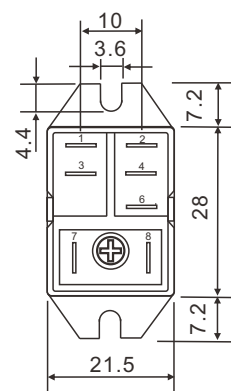
Flange Cover
