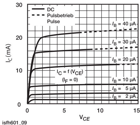
Fig. 9 - Transistor Characteristics
