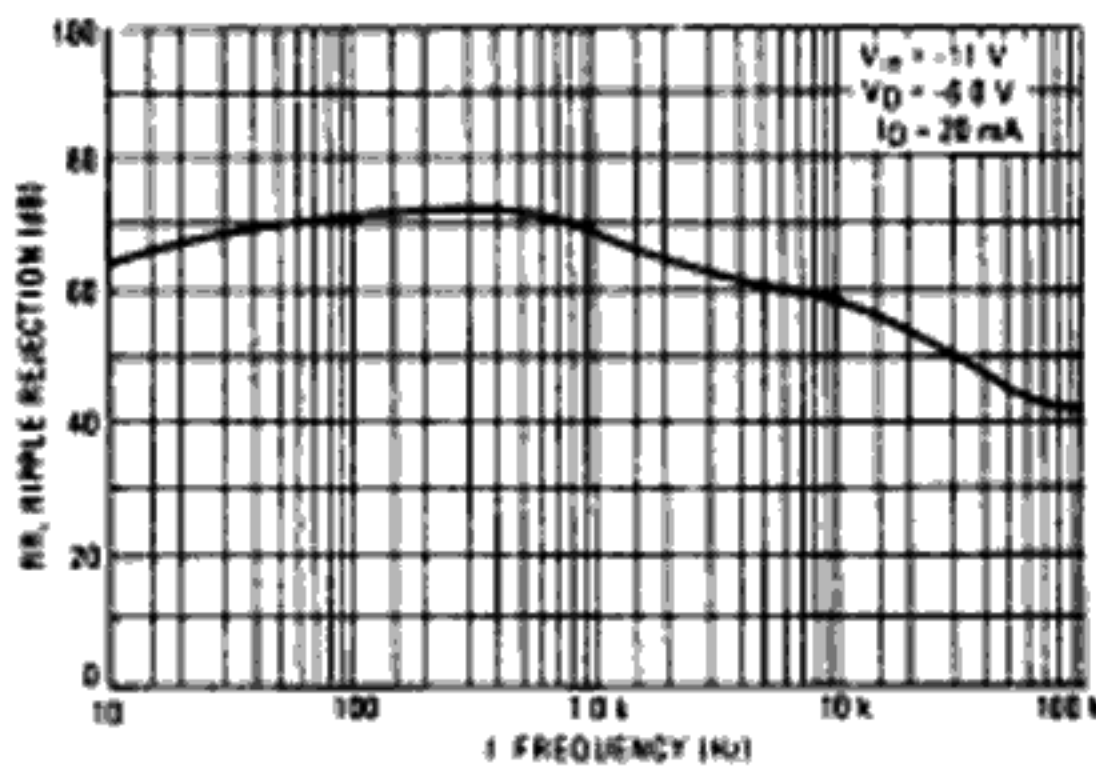
FIGURE 3 – RIPPLE REJECTION AS A FUNCTION OF FREQUENCY
