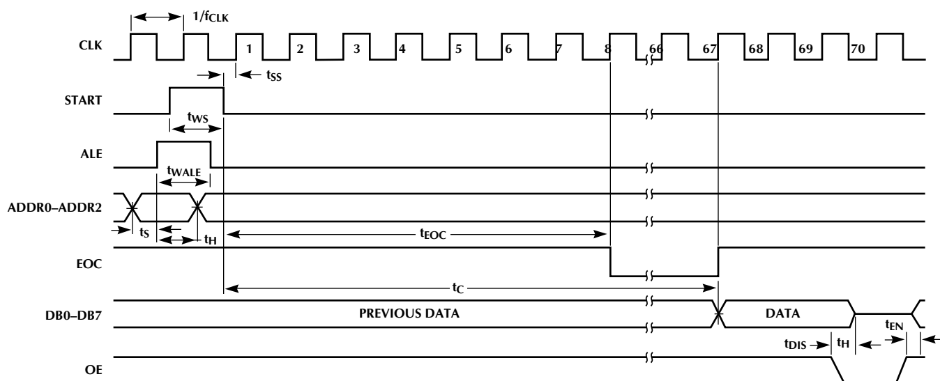
Figure 5. Timing Diagram
