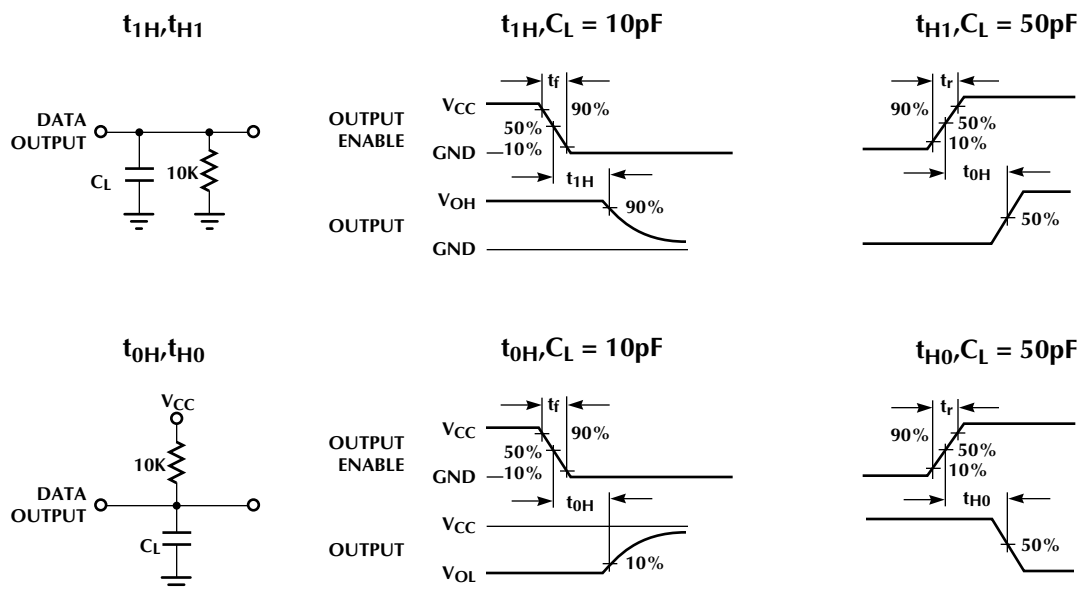
Figure 1. High Impedance Test Circuits and Waveforms
