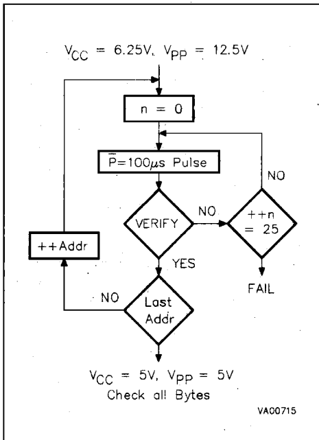
Figure 7. Programming Flowchart
