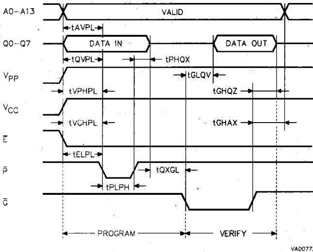
Figure 6. Programming and Verify Modes AC Waveforms
