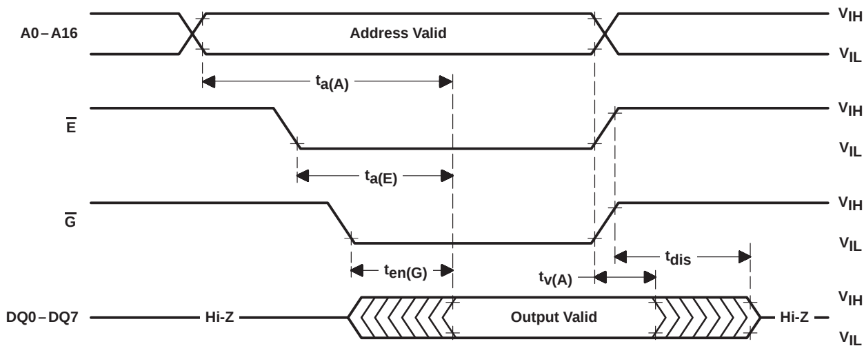
Figure 3. Read-Cycle Timing
