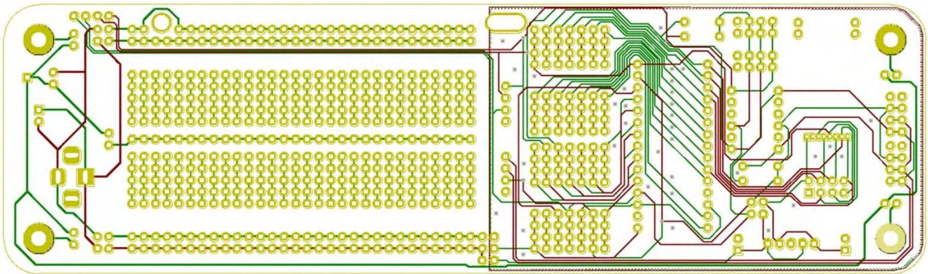
Figure 12: Electrical connections of the Proto-N2RF .
