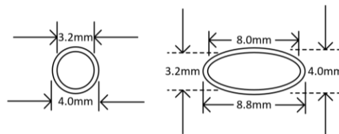
Figure 11: Dimensions of circular LCD mounting hole (left) and oval LCD mounting hole (right).
