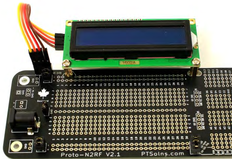
Figure 15: Mounting a common LCD module to the Proto-N2RF .
