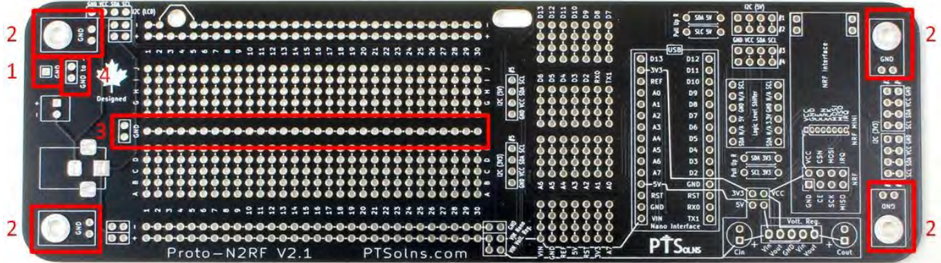
Figure 3: Various GND connection options of the Proto-N2RF. 1) GND out pin, 2) GND of each of the four mounting holes, 3) GND of the central rail, 4) GND to negative terminal connection.
