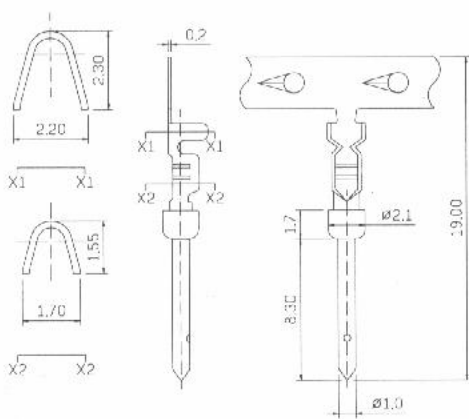
1.0 Crimp Pin Male
