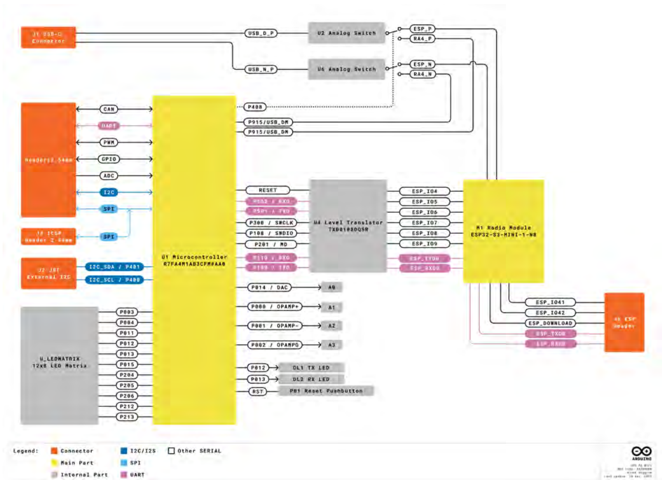
Arduino R4 WiFi Block Diagram
