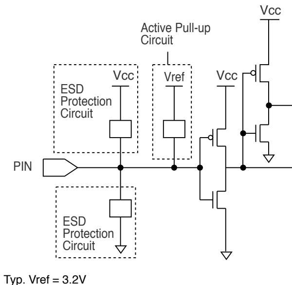
Typical Input
