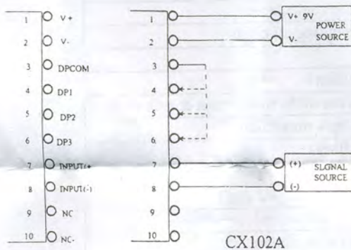
Wiring Diagram for CX102A (9V independent P/S)
