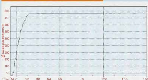
SIA Heating curve determination:
